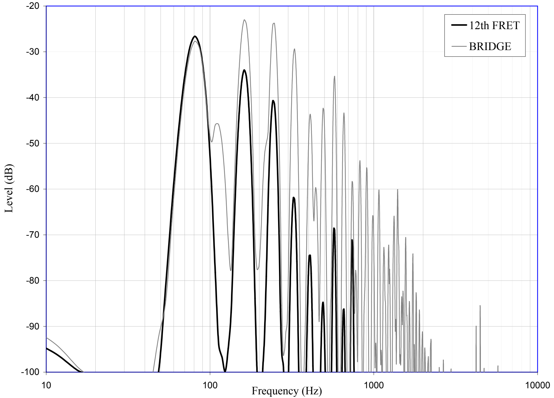
Frequency analysis of a plucked 'E' string on an electric guitar - recorded using magnetic pickup
