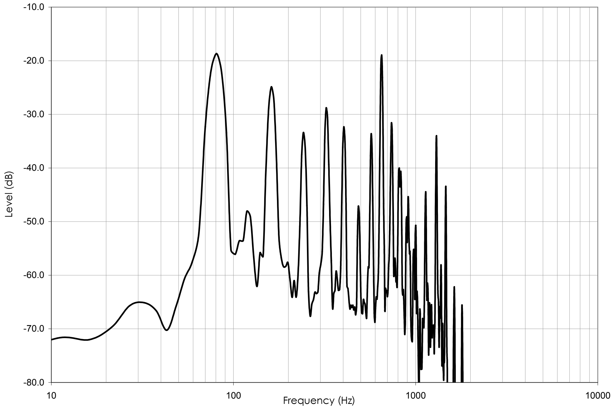
Frequency analysis of a single bass note from the 'Doctor Who' theme
